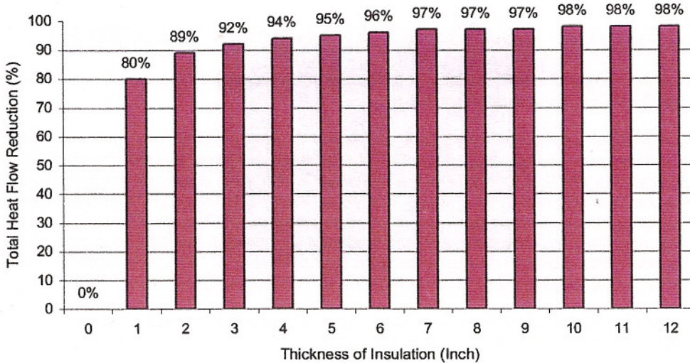
Figure 1.2: Percentage of total heat flow reduction
